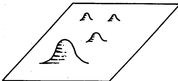
Figure 2. Multi-paradigm model
